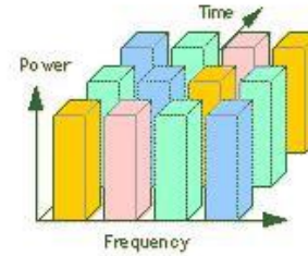
Figure 1. TDMA
