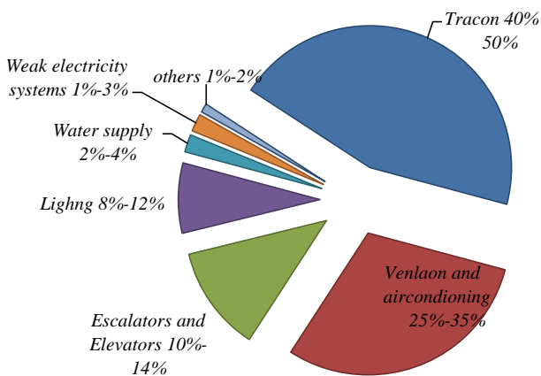
Fig. 3 Distribution of energy consumption in urban rail transit systems [32]
