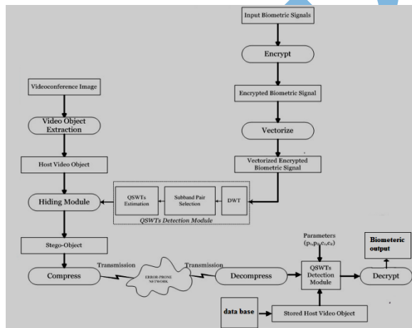
1.a): Remote Authentication activity diagram.
